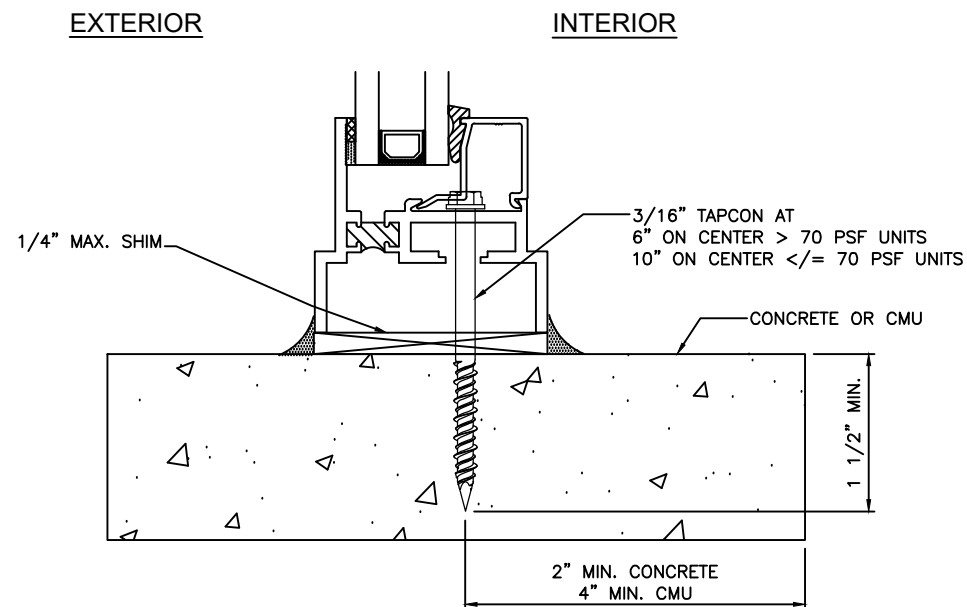
SECTION 1/1, 1/2 & 1/3 THROUGH FRAME TO CONCRETE OR CMU
