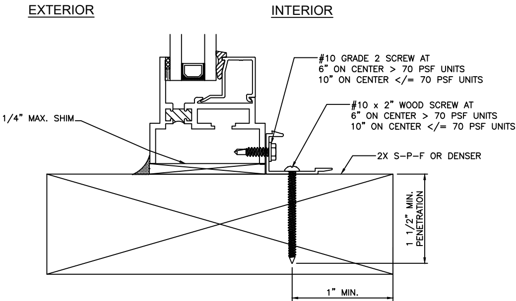
SECTION 1/1, 1/2 & 1/3 INSIDE CLIP & ANCHOR TO WOOD FRAME OR BUCK
