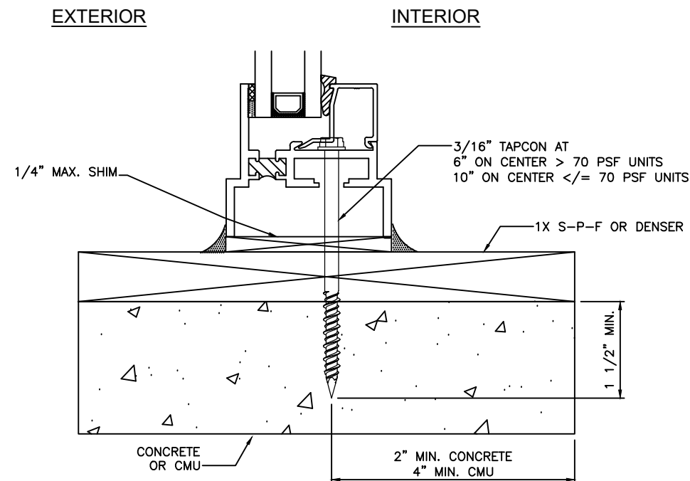
SECTION 1/1, 1/2 & 1/3 THROUGH FRAME TO CONCRETE OR CMU WITH 1X BUCK STRIP
