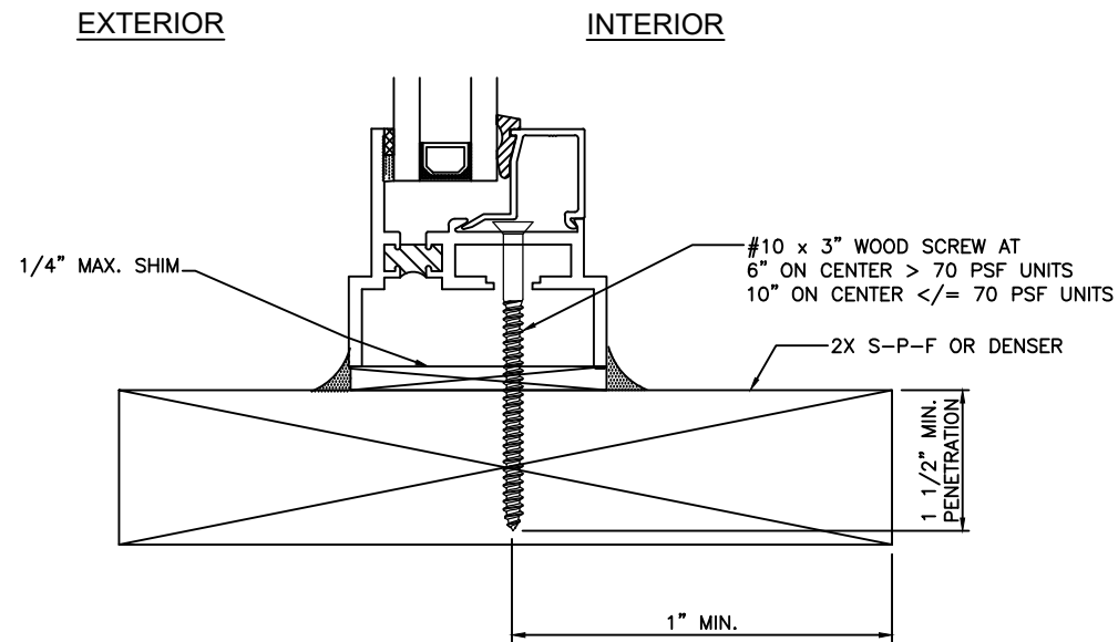
SECTION 1/1, 1/2 & 1/3 THROUGH FRAME TO WOOD FRAMING OR BUCK
