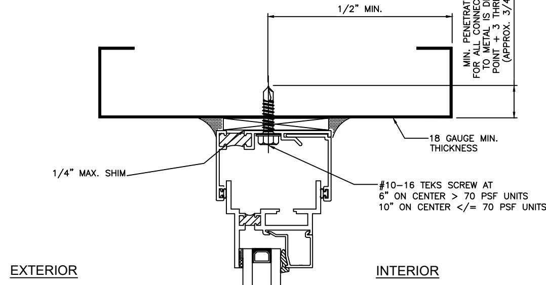
SECTION 1/1, 1/2 & 1/3 RECEPTOR TO STEEL STUD SUBSILL SIMILAR
