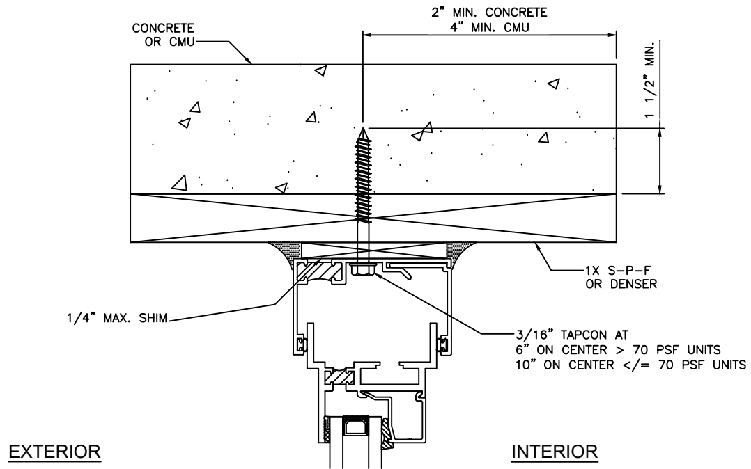
SECTION 1/1, 1/2 & 1/3 RECEPTOR TO CONCRETE OR CMU WITH 1X BUCK STRIP SUBSILL SIMILAR
