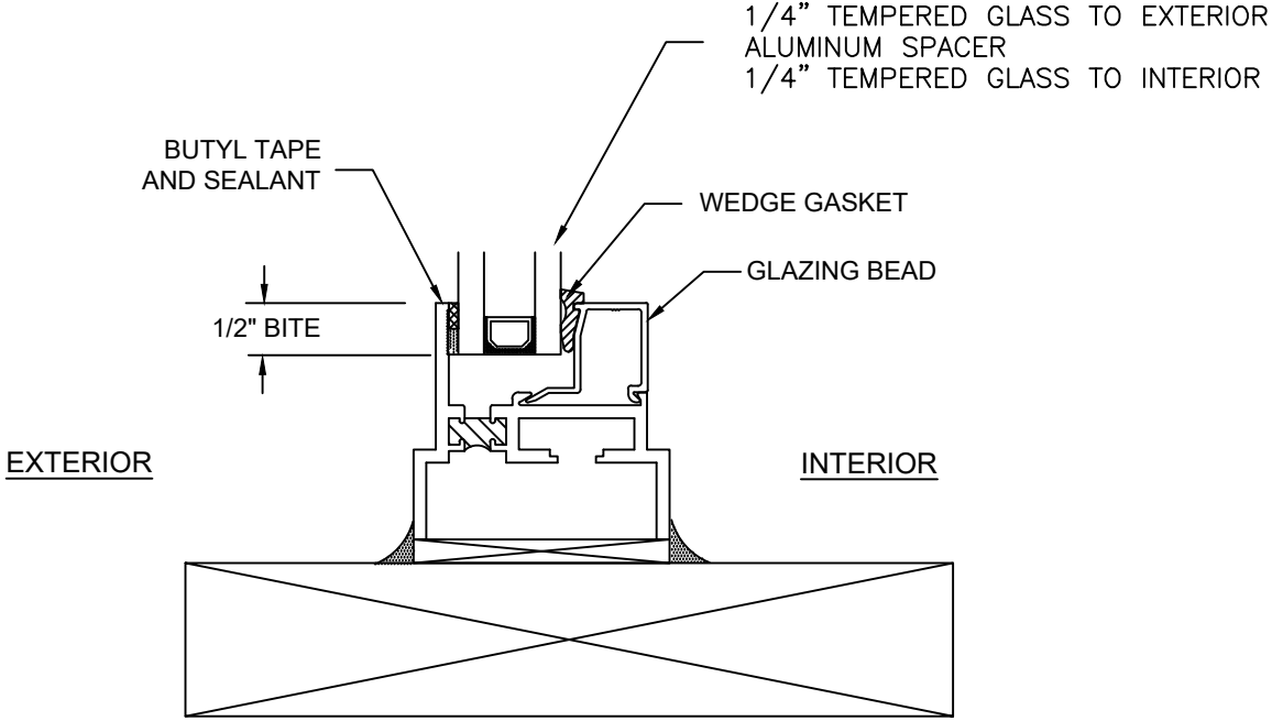
INSULATING GLASS GLAZING DETAIL
