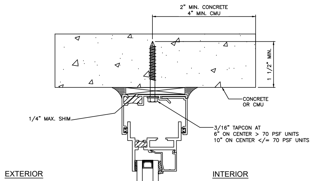
SECTION 1/1, 1/2 & 1/3 RECEPTOR TO CONCRETE OR CMU SUBSILL SIMILAR
